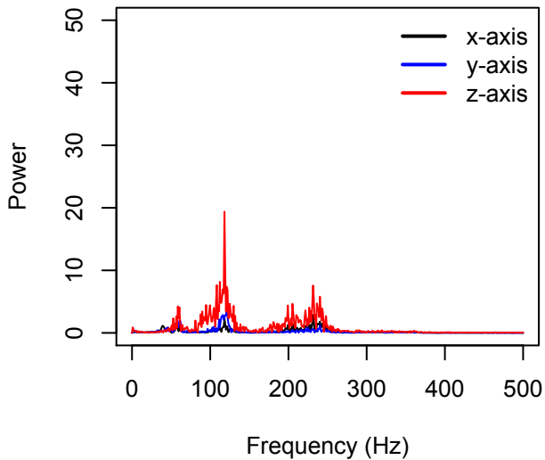
Accelerometer 1
