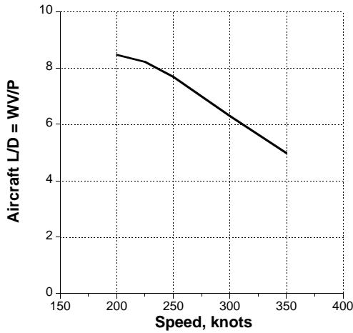
Fig. 14 Aircraft lift-to-drag ratio.
