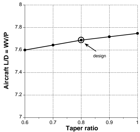
Fig. 18 Effect of blade taper on performance.
